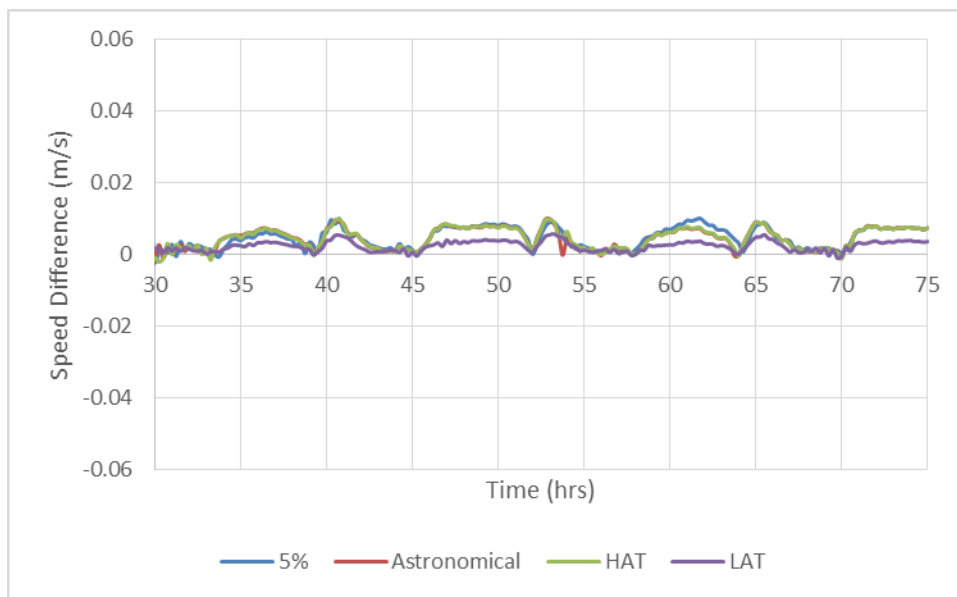
Figure 5-6 - P11 timeseries: Near East – Comparison between Baseline and Scheme scenarios
