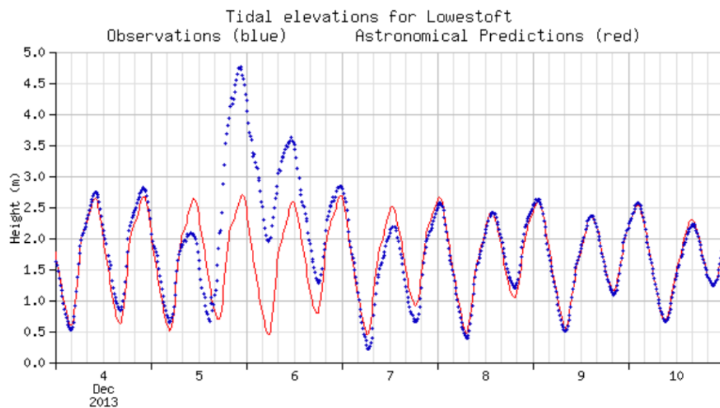
Figure 4-6 - Levels (mCD) at Lowestoft Gauge. (National Tidal and Sea Level Facility website, extracted 2016)
