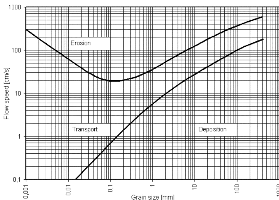
Figure 5-2 - Hjulström Curve
