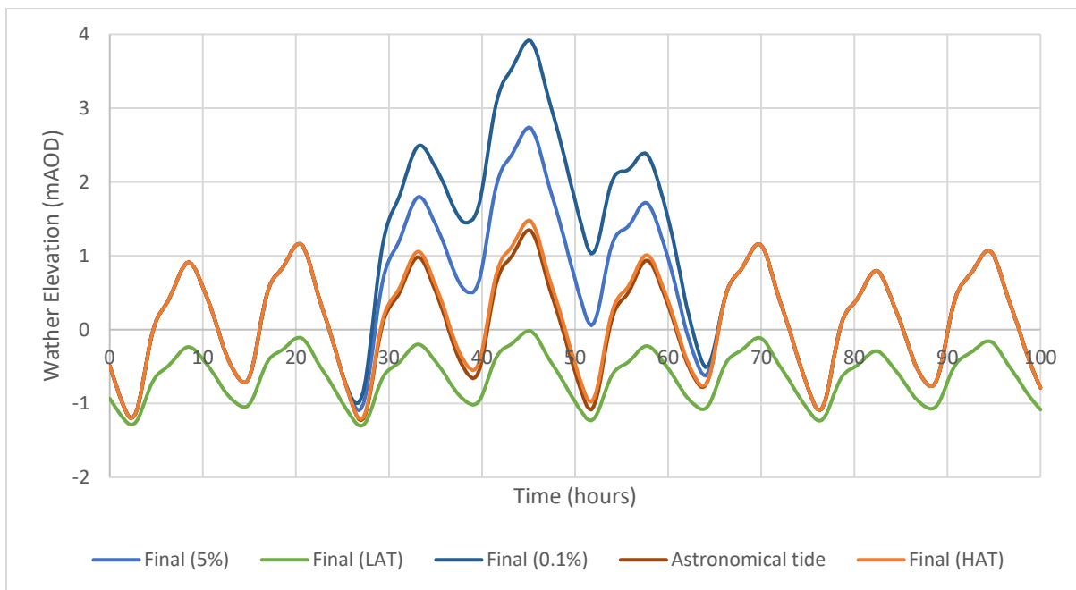
Figure 3-1 - Tidal curve for 5% AEP, LAT, 0.1% AEP, Astronomical and HAT present day events
