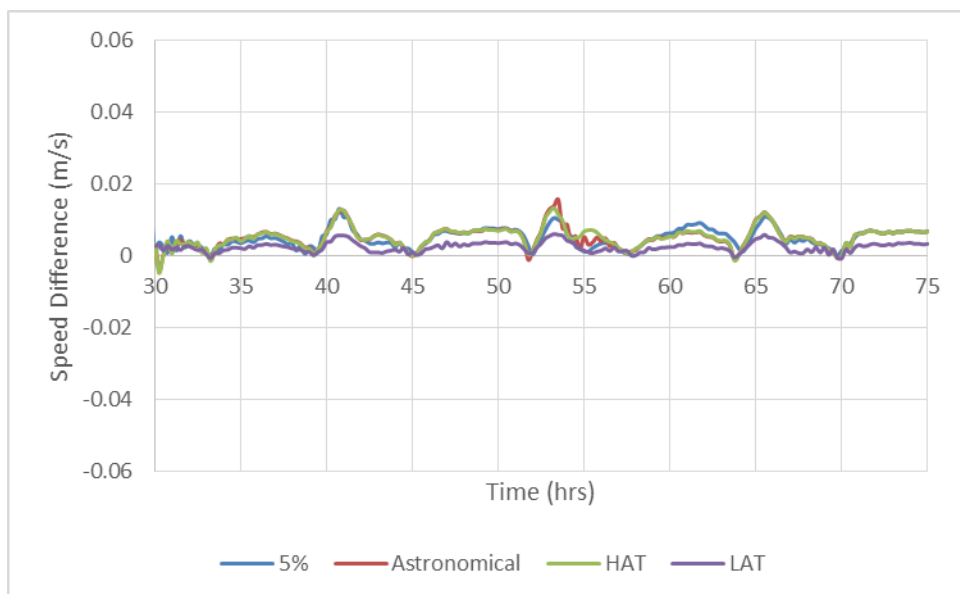
Figure 5-5 - P6 timeseries: Near West – Comparison between Baseline and Scheme scenarios
