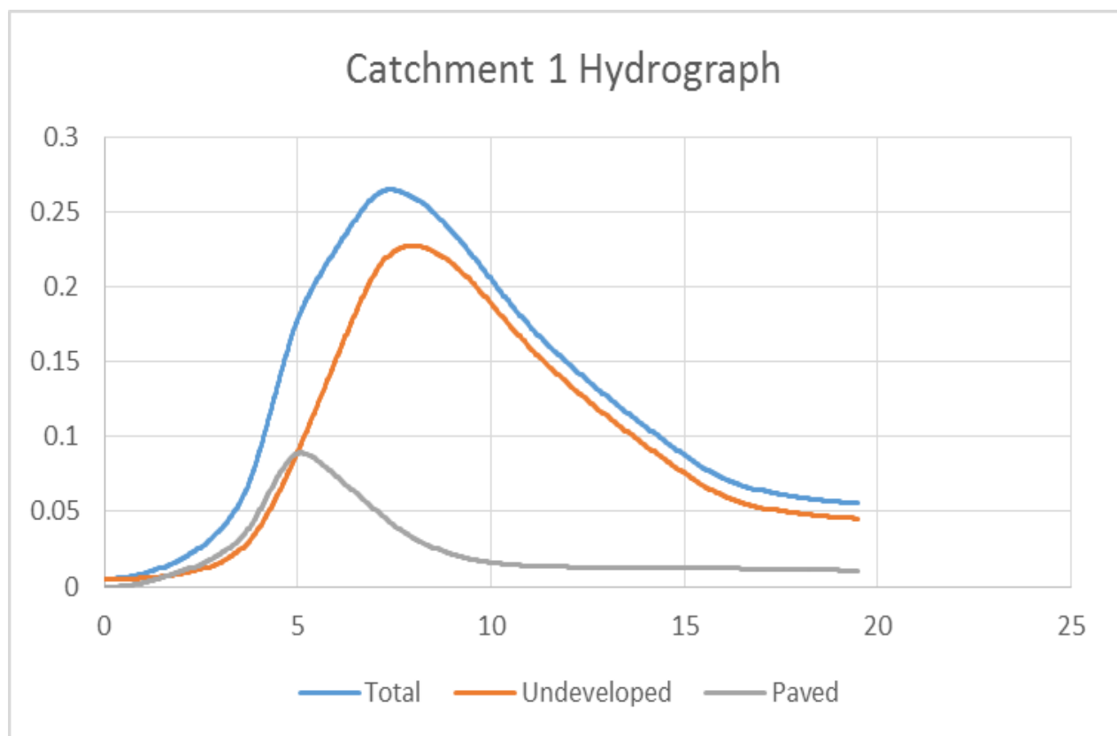
Figure B2, Catchment 1 Hydrograph
