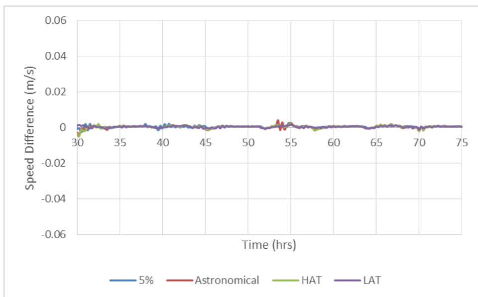
Figure 5-4 - P1 timeseries: Far west – Comparison between Baseline and Scheme scenarios
