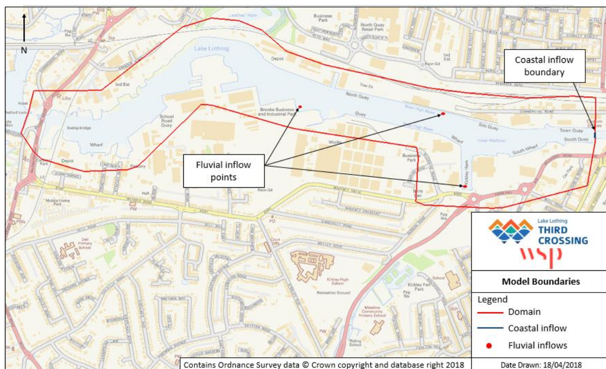
Figure 4-4 - Model boundary conditions
