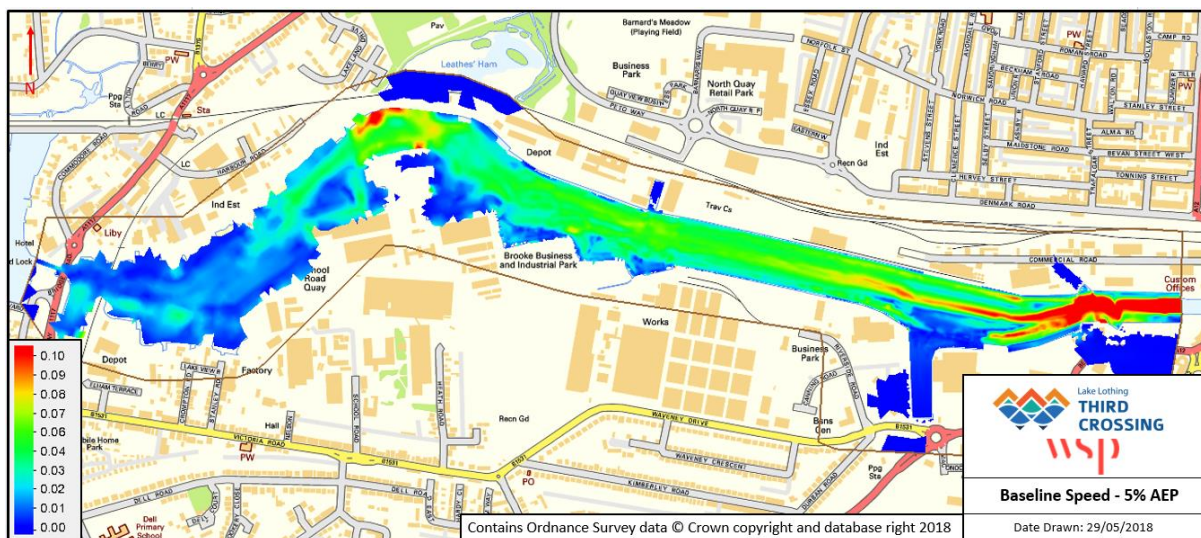
Figure 5-3 - Baseline Water Speed 5% AEP event
