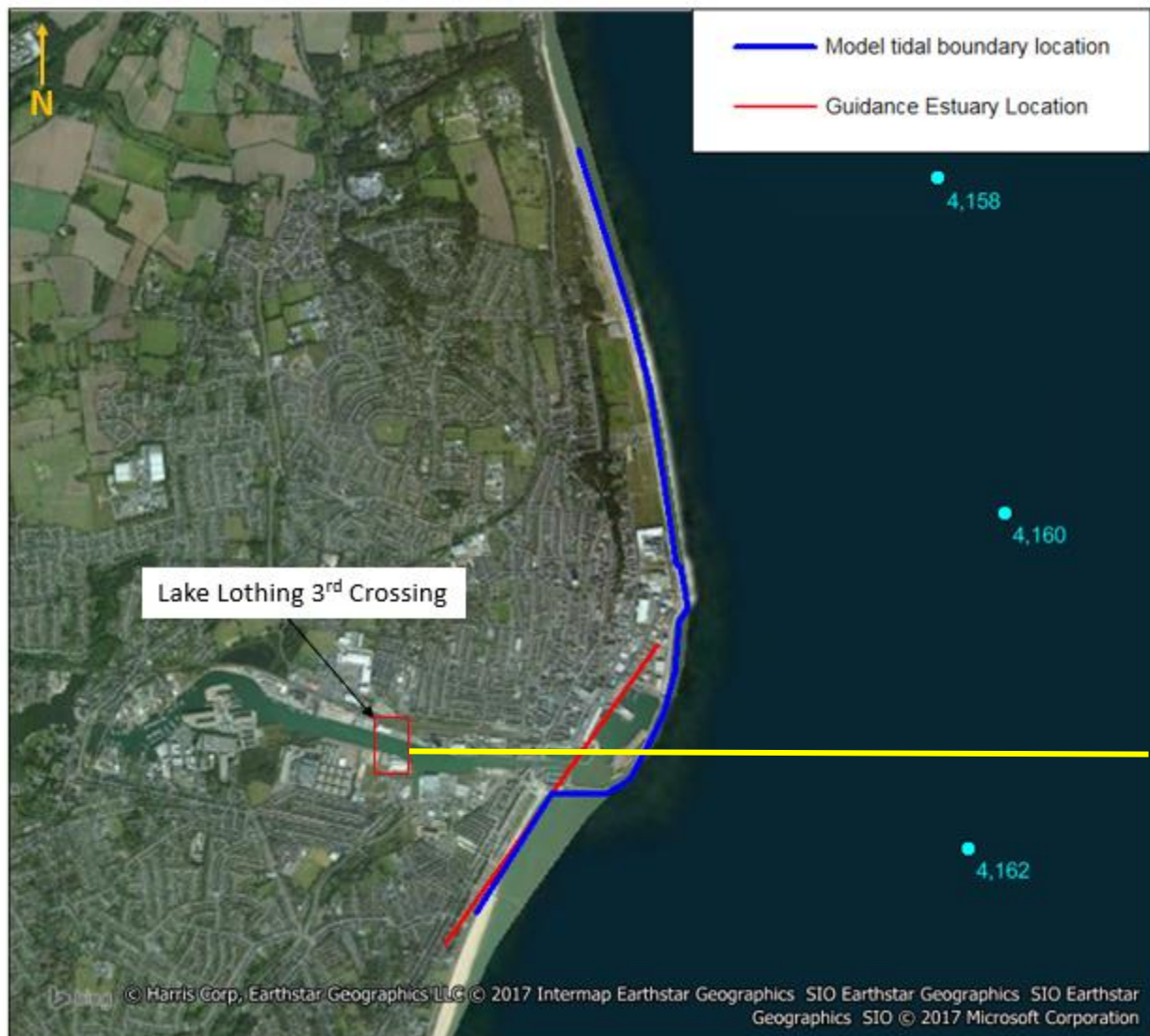
Figure 1: Estuary Boundary Check
