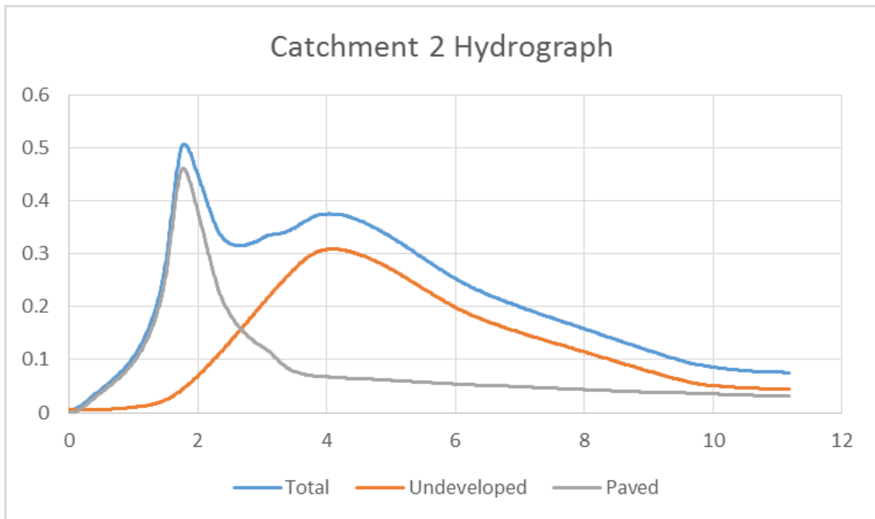
Figure B3, Catchment 2 Hydrograph
