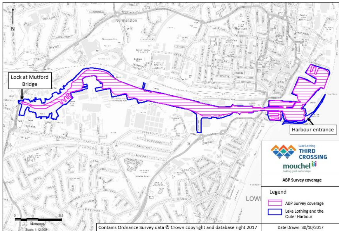
Figure 4-3 - ABP bathymetric survey coverage in Lake Lothing
