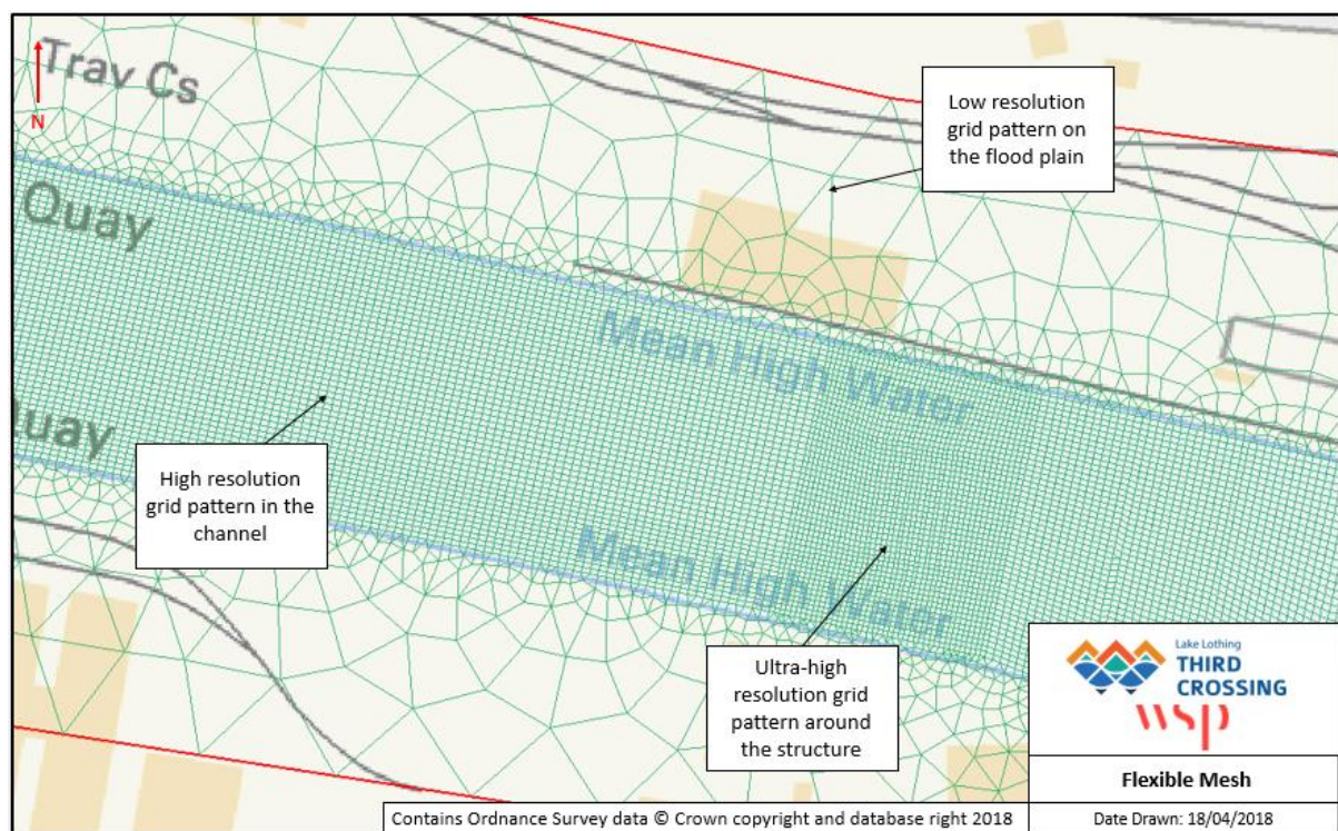
Figure 4-2 – Flexible mesh
