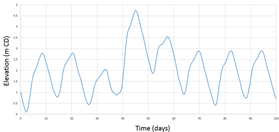
Figure 4-7 - 2013 event tidal curve
