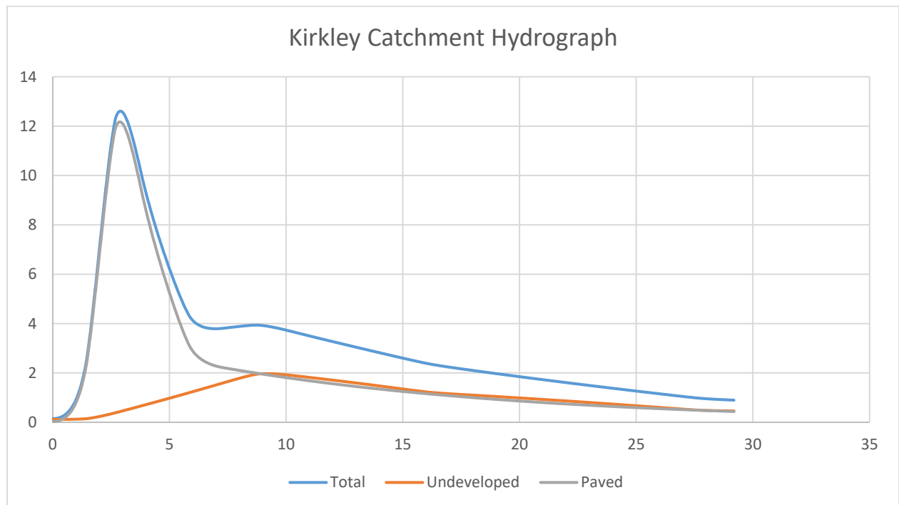
Figure B1, Kirkley stream hydrograph
